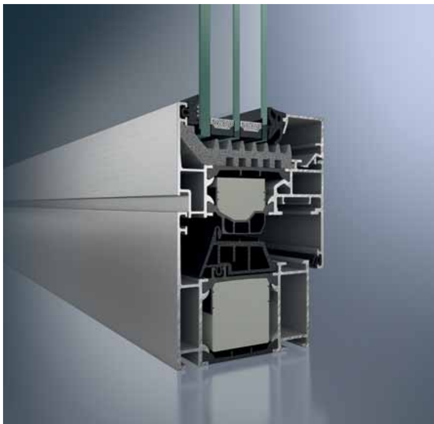
The super-insulated Schueco AWS 75.SI+ window with triple-glazing
